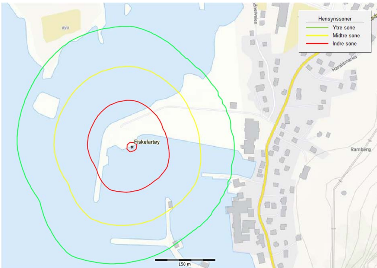
Figur 17 Beregnede hensynssoner for ammoniakk – Ramberg
