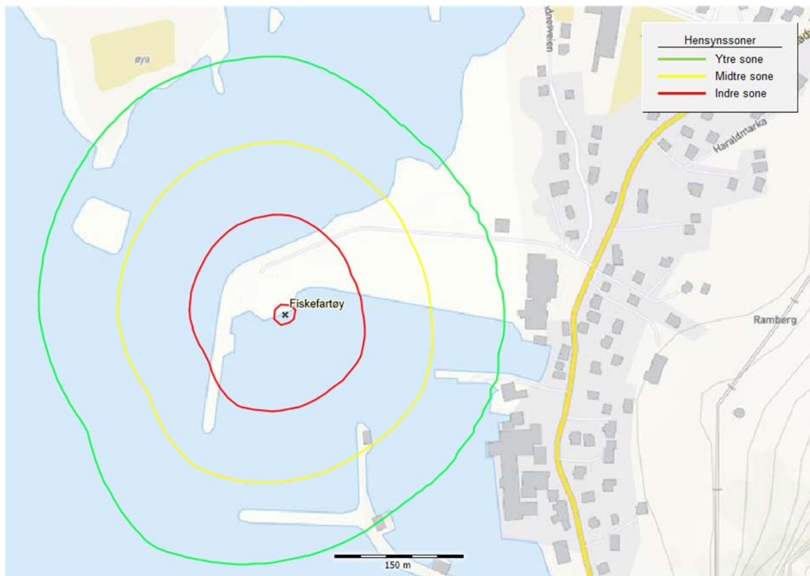
Figur 5-6 Beregnede hensynssoner for ammoniakk – Ramberg
